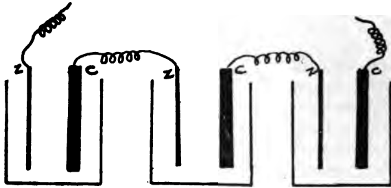
FIG. 276.—Diagram of a Series Circuit, showing Three Galvanic Cells in Battery. As shown, the copper, or positive, pole of the first cell is connected to the zinc, or negative, pole of the second, and so on; leaving a negative terminal at one end and a positive at the other. Thus the current emerging from each cell passes through all those succeeding in line, the total voltage of the battery being equivalent to the sum of the individual voltages of the several cells. If, on the other hand, several motors, or other electrically affected apparatus, be connected in series, the result is to increase the "back pressure" (C. E. M. F.) on the same ratio, and hence cut down the operative efficiency of each.
